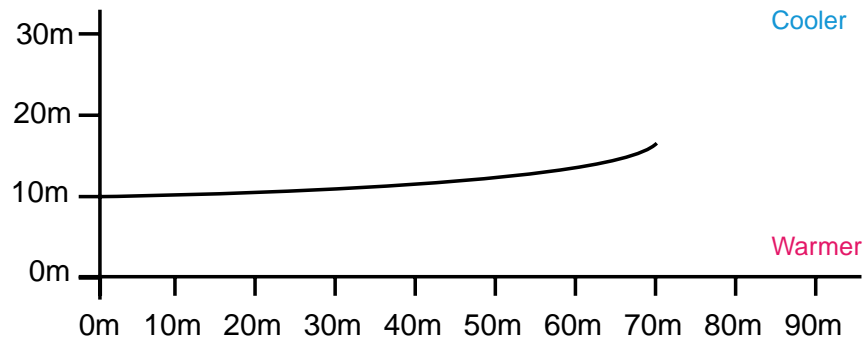
Sound path tilting upwards outdoors due to normal temperature decrease with height
