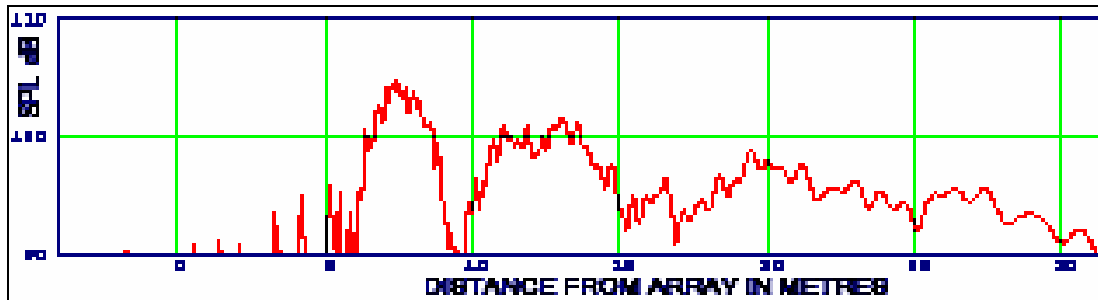
Irregular coverage from a J-Shaped Array
